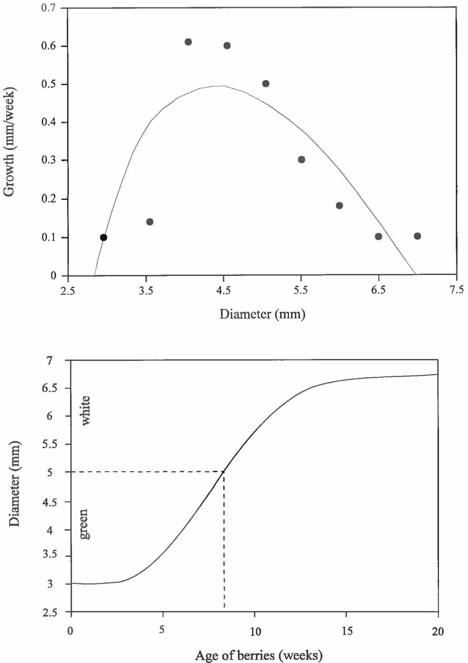
Figure 15. Growth rate of Pukiawe berries in relation to their size (Kau Desert) y=0.37-0.37/(x-0.47)^{(0.84-x)/(x-0.47)} 5.31 , N=9 , R^2=0.73 , after log-transformation of diameter). The integral form gives the size of berries in relation to age (bottom).
