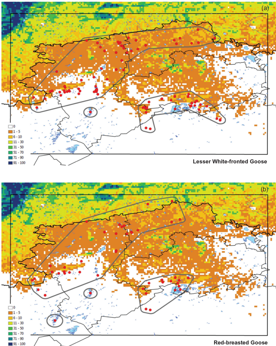
Figure 3. Known locations (red circles) of (a) Lesser White-fronted Geese, and (b) Red-breasted Geese and their core areas (polygons with grey lines) plotted on the extent of forest cover (given as %) in the region. The overall study area is indicated (rectangle), along with regional and national boundaries.
