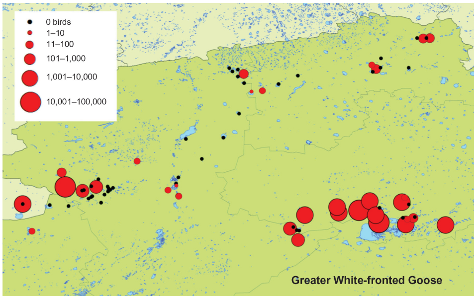
Figure 5. Location and numbers of Greater White-fronted Geese staging at lakes in northern regions of Kazakhstan and at Zhetyskol and Balakol Lakes in Russia during the autumn 2016 survey.
