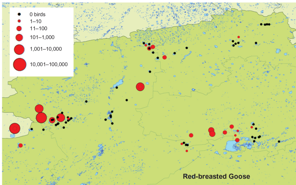
Figure 6. Location and numbers of Red-breasted Geese staging at lakes in northern regions of Kazakhstan and at Zhetyskol and Balakol Lakes in Russia during the autumn 2016 survey.
