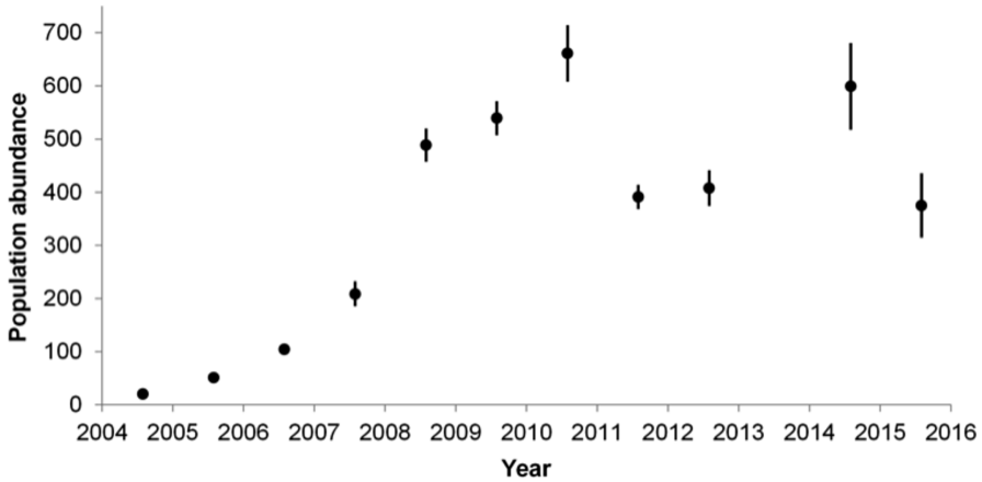
Figure 2. Modified Chapman bias-corrected Lincoln-Petersen mark-resightings population abundance estimates with 95% confidence intervals (CI) for Laysan Teal at Midway Atoll, Hawai'i, for the years 2007–2015. Before 2007 all adults were given radio transmitters, so the abundance was known exactly for those 3 years. No abundance estimate was generated for 2013 because no surveys were undertaken in this calendar year.
